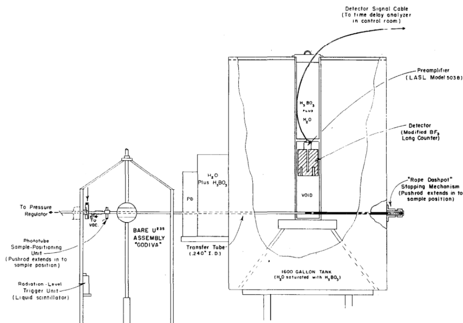
Figure 2.1: Experimental setup for measuring delayed neutron emission from irradiation of GODIVA on a sample recreated from [59].
