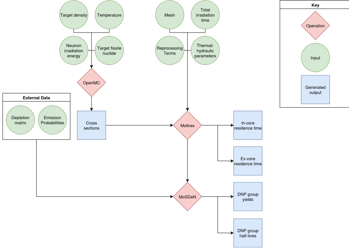
Figure 3.4: Flow diagram of spatially resolved flow model used to generate improved DNP group parameters.
