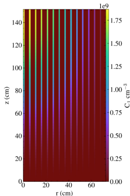
Figure 2: The longest-lived DNP group concentration in the 2D axisymmetric Moltres MSRE model from [17].
