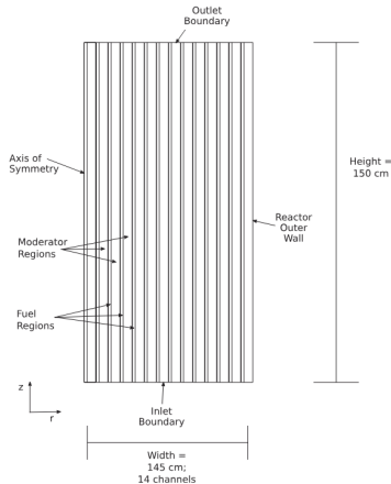
Figure 13: A sketch of the 2D MSRE Moltres model geometry (from [17]).
