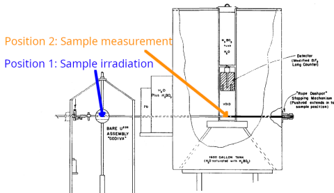
Figure 4: Simplified experimental setup for measuring delayed neutron emission from irradiation of a 3 gram sample in Godiva referenced from [15].
