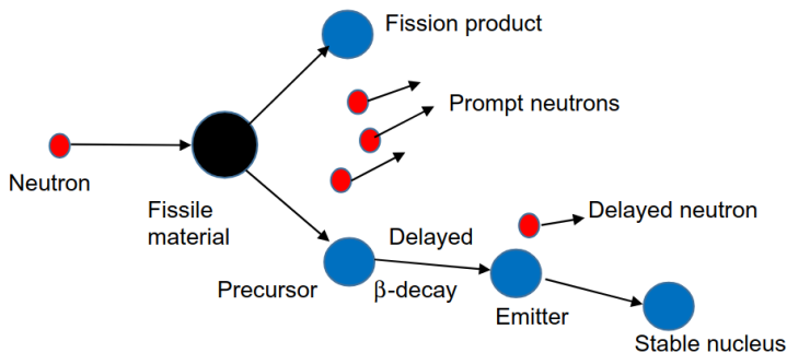
Figure 1: The process of delayed neutron emission from [16].
