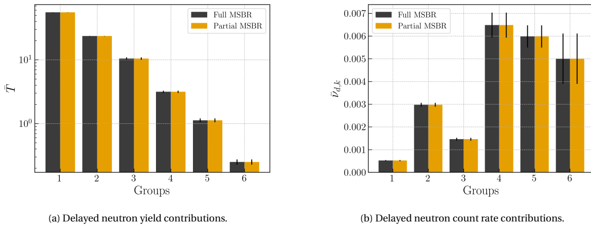
Figure 4.3: Delayed neutron contributions from each DNP.
