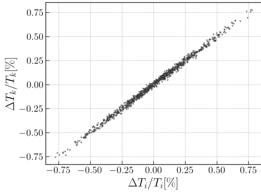
(c) DNP group 1 half-life variation due to half-life variation.
