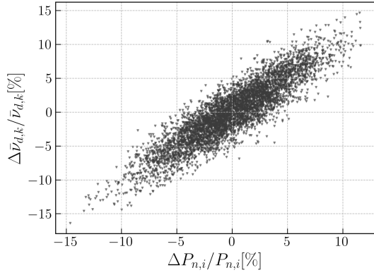
(a) DNP group 1 yield variation due to emission probability variation.
