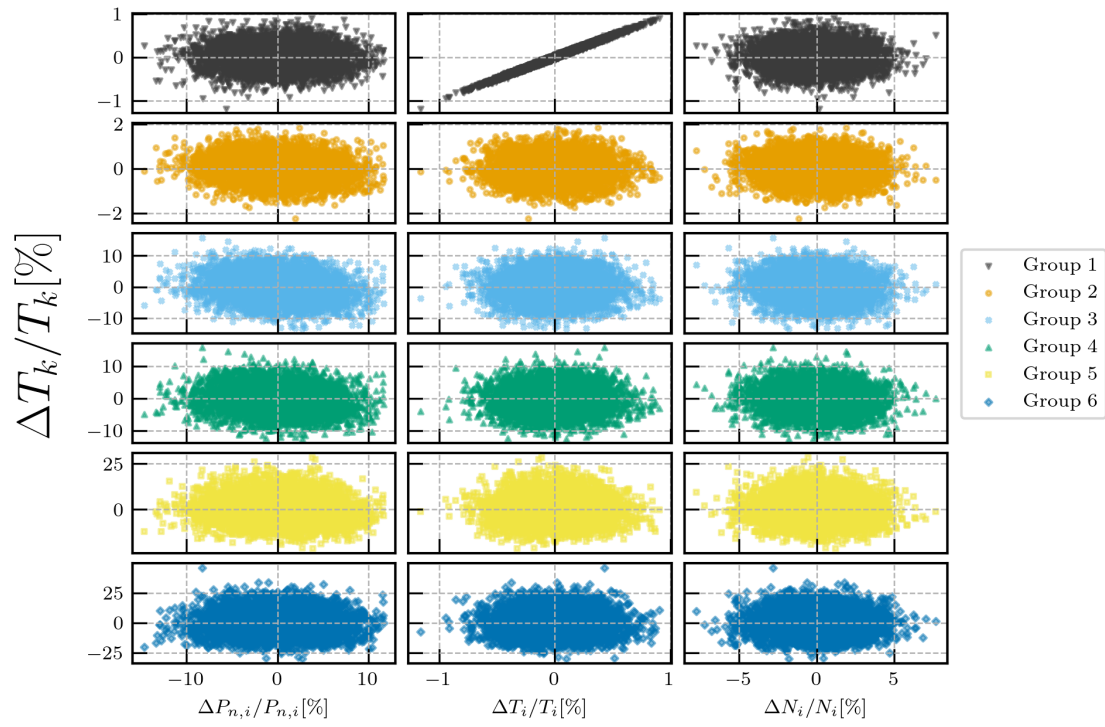
Figure 4.11: The difference in each DNP group half-life from the ^{87}\text{Br} relative changes in emission probability, half-life, and concentration.
