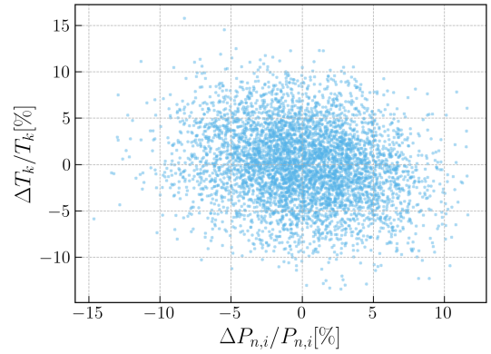
(d) DNP group 3 half-life variation due to emission probability variation.
