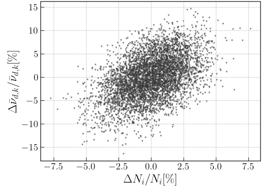
(b) DNP group 1 yield variation due to fission yield variation.
