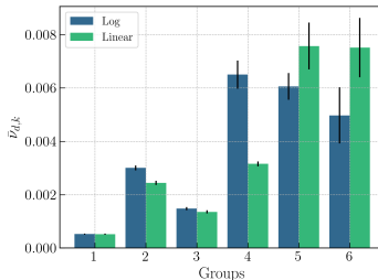
Figure 20: \bar{v}_{d,k} for each DNP group k after a thermal saturation irradiation of ^{235}\text{U} using the 0D scaled model.
