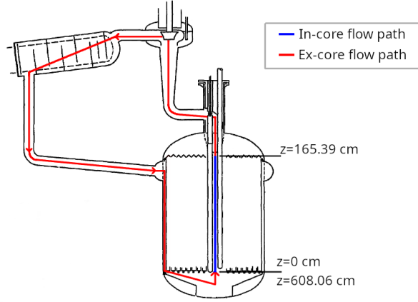
Figure 3.2: The flow path and bounds for the in-core region of the MSRE, overlaid on the MSRE loop diagram from [7].
