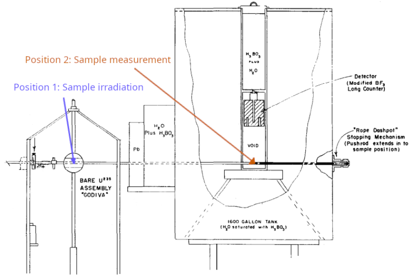
Figure 2.1: Simplified experimental setup for measuring delayed neutron emission from irradiation of a 3 gram sample in Godiva recreated from [? ].
