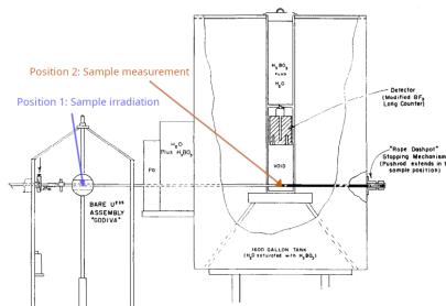
Figure 4: Simplified experimental setup for measuring delayed neutron emission from irradiation of a 3 gram sample in Godiva referenced from [16].
