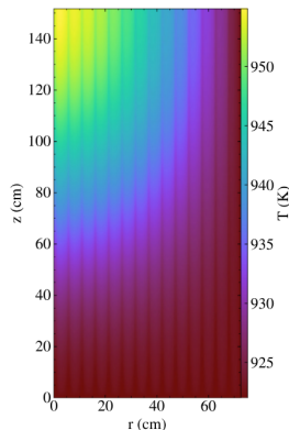
Figure 2: The temperature profile in the 2D axisymmetric Moltres MSRE model from [18].
