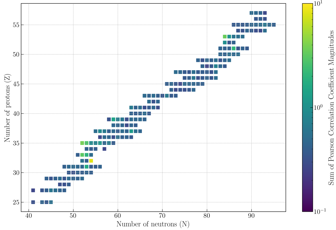
Figure 4.14: The sum of the PCC magnitudes for each DNP on each group half-life \tau_k and yield \bar{v}_{d,k} after a thermal saturation irradiation of ^{235}\text{U} using the 0D scaled model. The ^{86}\text{Ge} summed value is noticeably larger than the others, indicating its uncertainties have a larger impact on group parameters than other DNPs.
