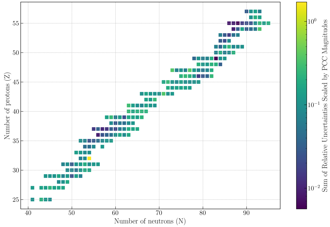
Figure 4.15: The sum of the PCC magnitudes times the relative uncertainties for each DNP on each group half-life \tau_k and yield \bar{v}_{d,k} after a thermal saturation irradiation of ^{235}\text{U} using the 0D scaled model. The ^{86}\text{Ge} summed value is slightly larger than the others, though there are many DNPs which can use improved data.
