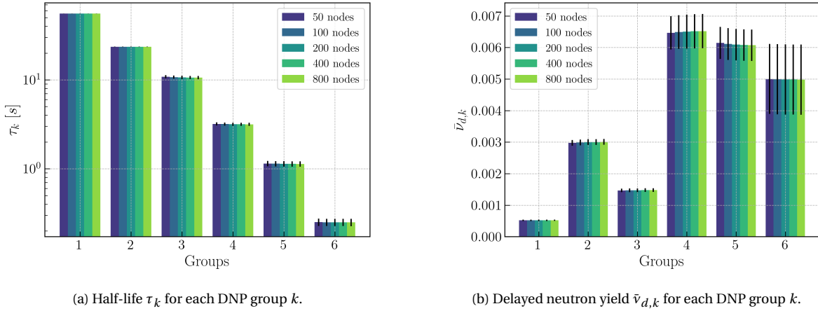
Figure 4.6: DNP group parameters for varying numbers of time nodes after a thermal saturation irradiation of ^{235}\text{U} using the 0D scaled model. Increasing the number of nodes increases the accuracy of the DNP group parameters, with differences in the yields that are within uncertainty bounds.
