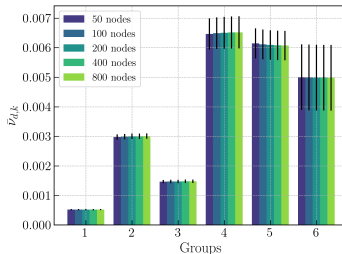
Figure 22: \bar{v}_{d,k} for each DNP group k after a thermal saturation irradiation of ^{235}\text{U} using the 0D scaled model.
