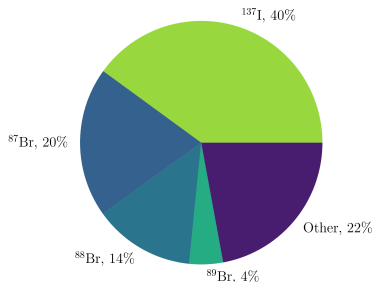
Figure 8: Relative delayed neutron counts from each DNP after a thermal saturation irradiation of ^{235}\text{U} using the 0D scaled model.
