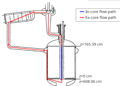
Figure 5: The flow path and bounds for the in-core region of the MSRE, overlaid on the MSRE loop diagram from [10].
