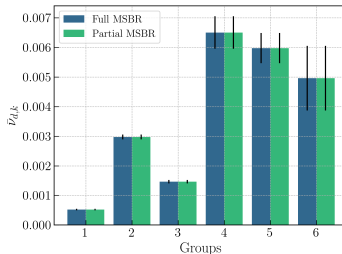
Figure 16: \bar{v}_{d,k} for each DNP group k after a thermal saturation irradiation of ^{235}\text{U} using the 0D scaled model.
