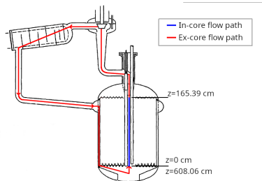
Figure 3: The flow path and bounds for the in-core region of the MSRE, overlayed on the MSRE loop diagram from [10].
