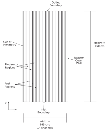
Figure 11: A sketch of the 2D MSRE Moltres model geometry (from [19]).
