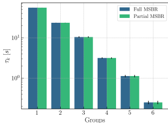
Figure 13: \tau_k for each DNP group k after a thermal saturation irradiation of ^{235}\text{U} using the 0D scaled model.
