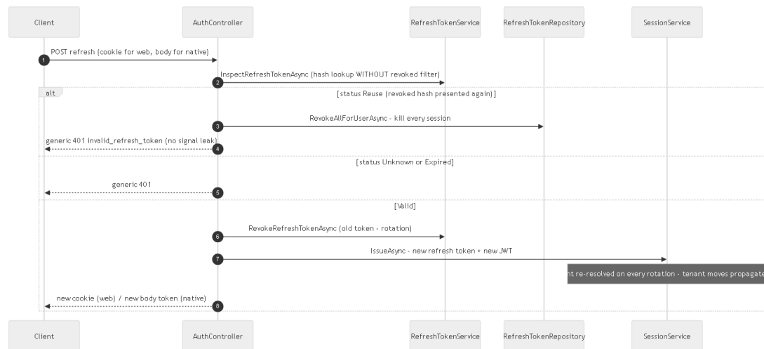
Figure 2.2 · Refresh rotation &amp; reuse detection — the flow you just ran (FLOWS.md §7)
