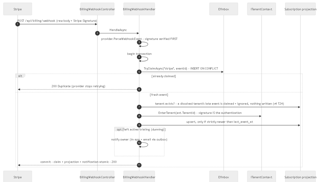
Figure 5.2 · The billing webhook — Stripe event to subscription projection (FLOWS.md §8)
