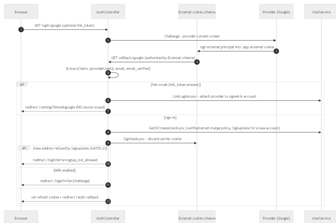
Figure 2.5 · The OAuth (web) sign-in dance (FLOWS.md §5)
