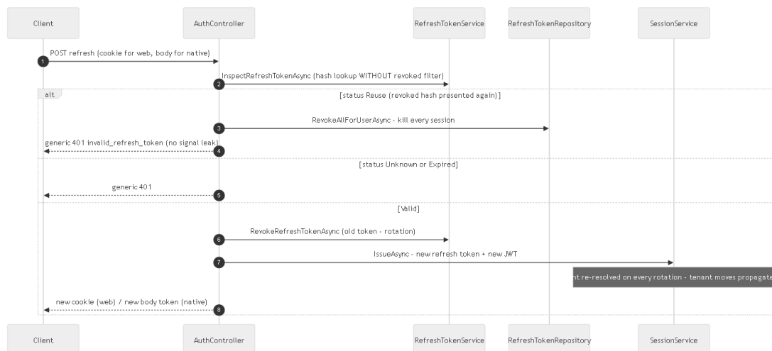
Figure 2.2 · Refresh rotation & reuse detection — the flow you just ran (FLOWS.md §7)
