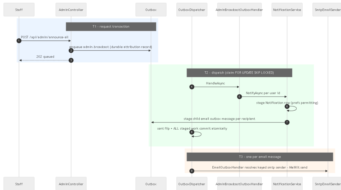
Figure 7.5 · Announce-all — three transactions, one outbox fan-out (FLOWS.md §9)
