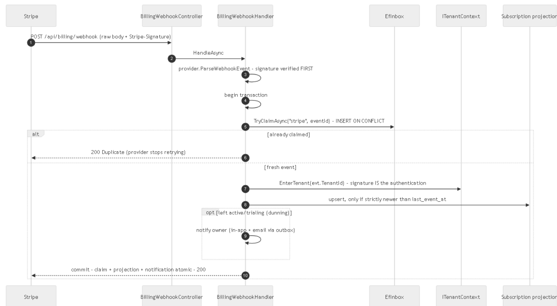
Figure 5.2 · The billing webhook — Stripe event to subscription projection (FLOWS.md §8)
