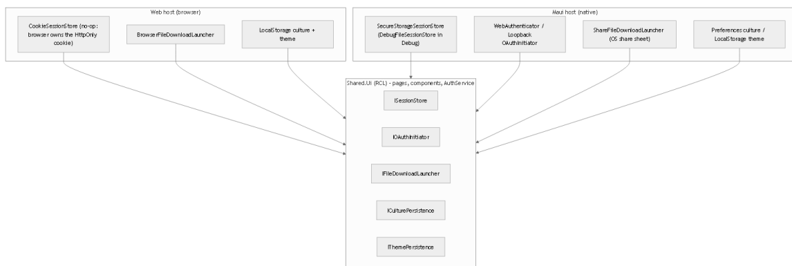
The shells' shared client architecture (ARCHITECTURE.md §9)
