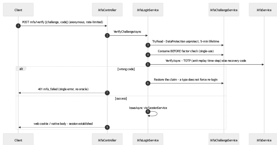
Figure 6.5 · MFA step-up completion — one choke point for every sign-in path (FLOWS.md §6)
