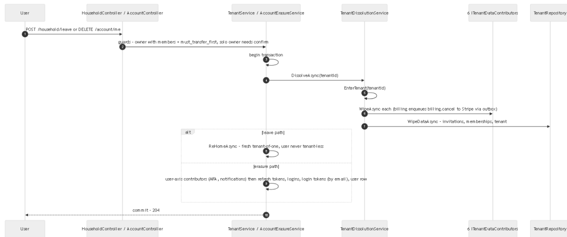
Figure 2.9 · Household dissolve — leave &amp; erasure through the contributor seam (FLOWS.md §11)
