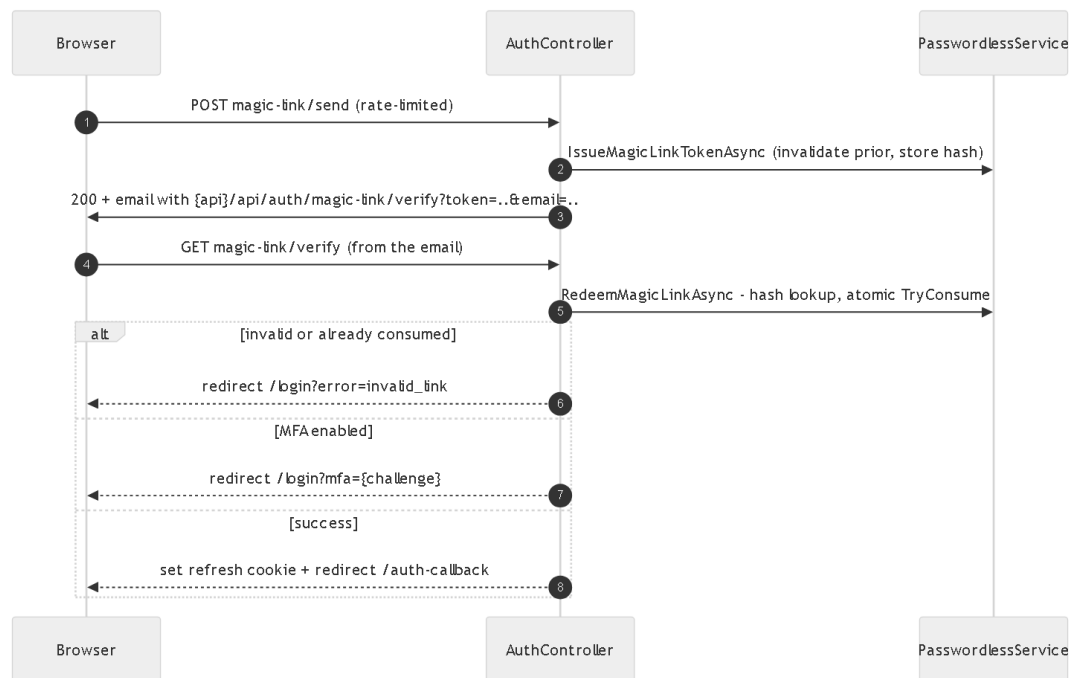
Figure 2.4a · Magic-link sign-in, end to end (FLOWS.md §4)
