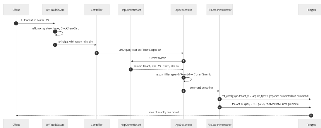
Figure 2.6 · An authenticated, tenant-scoped request — the filter in the call stack (FLOWS.md §2)
