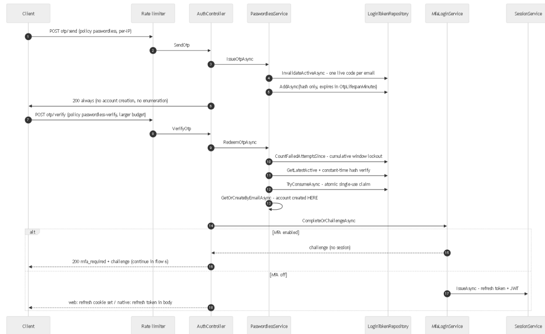
Figure 2.4b · Email OTP sign-in, end to end (FLOWS.md §3)
