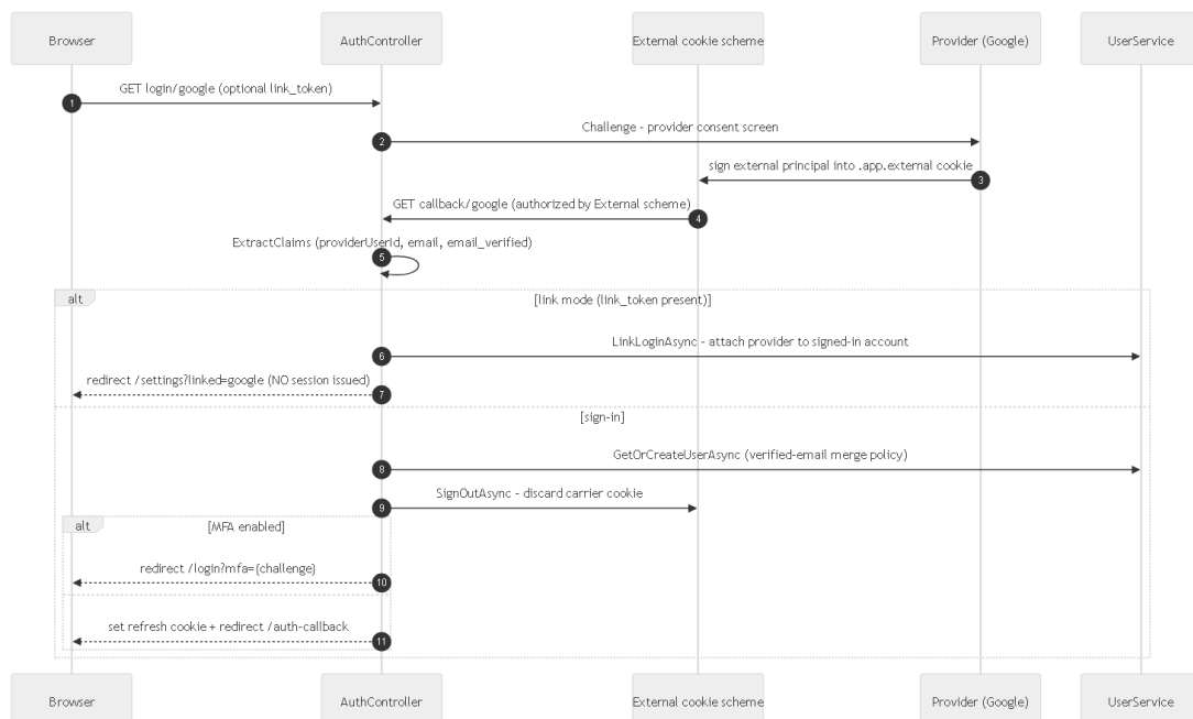
Figure 2.5 · The OAuth (web) sign-in dance (FLOWS.md §5)
