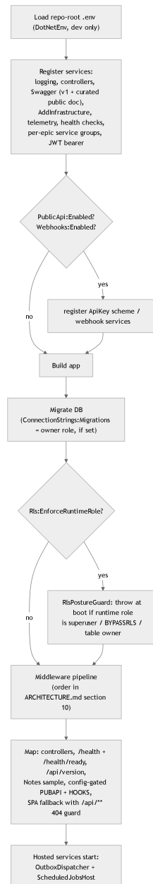
Figure 8.4 · The boot order — where migrations and the posture guard sit (FLOWS.md §1)
