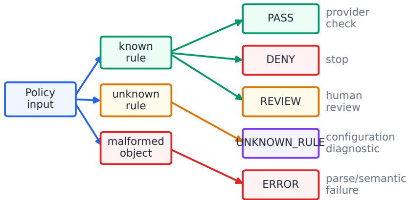
Figure 3. Typed policy lattice v0.2
