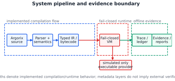
Fig. 1. Implemented source-to-evidence path. Metadata that reaches the trace is not thereby authenticated by an external authority.
