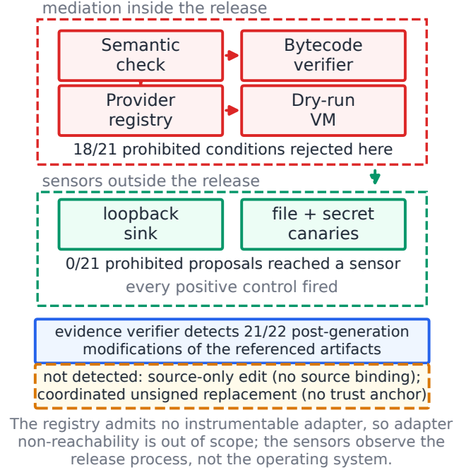
Fig. 2. Measured adversarial boundary. Counts are generated from the campaign summary, not transcribed. Rejection happens inside the release; the sensors that decide whether an effect escaped are outside it.
