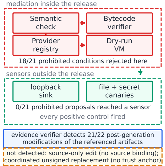
The registry admits no instrumentable adapter, so adapter non-reachability is out of scope; the sensors observe the release process, not the operating system.
