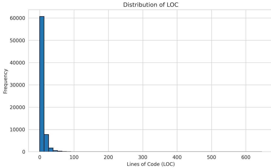
Figure 3. LOC Histogram
