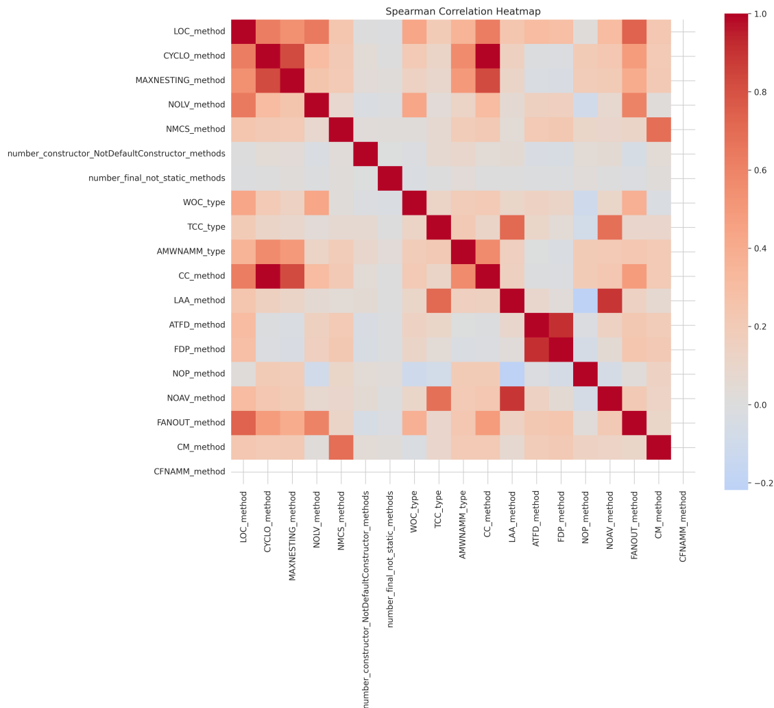
Figure 5. Metric Heatmap
