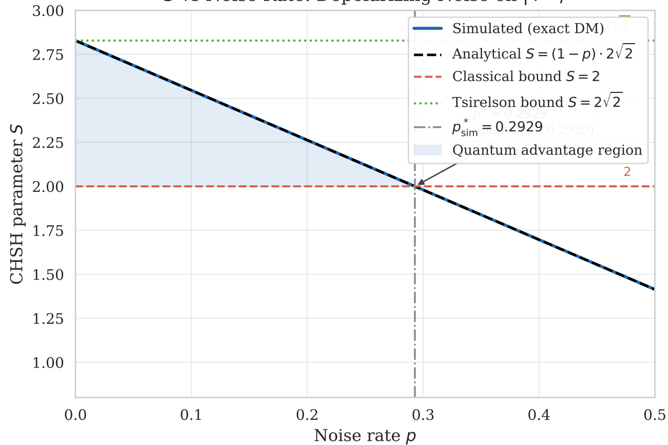
S vs Noise Rate: Depolarizing Noise on |\Phi^+\rangle
