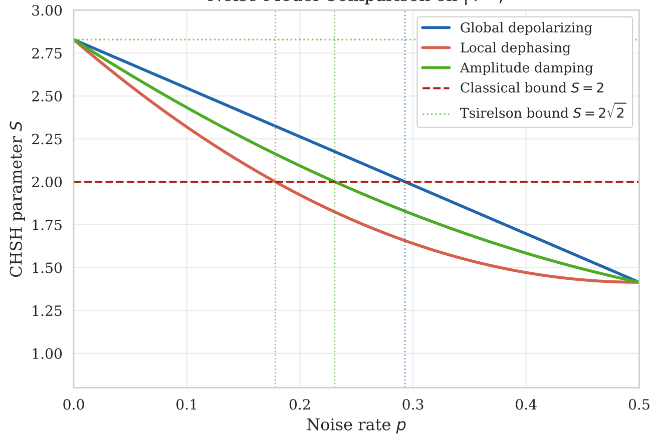
Noise Model Comparison on |\Phi^+\rangle
