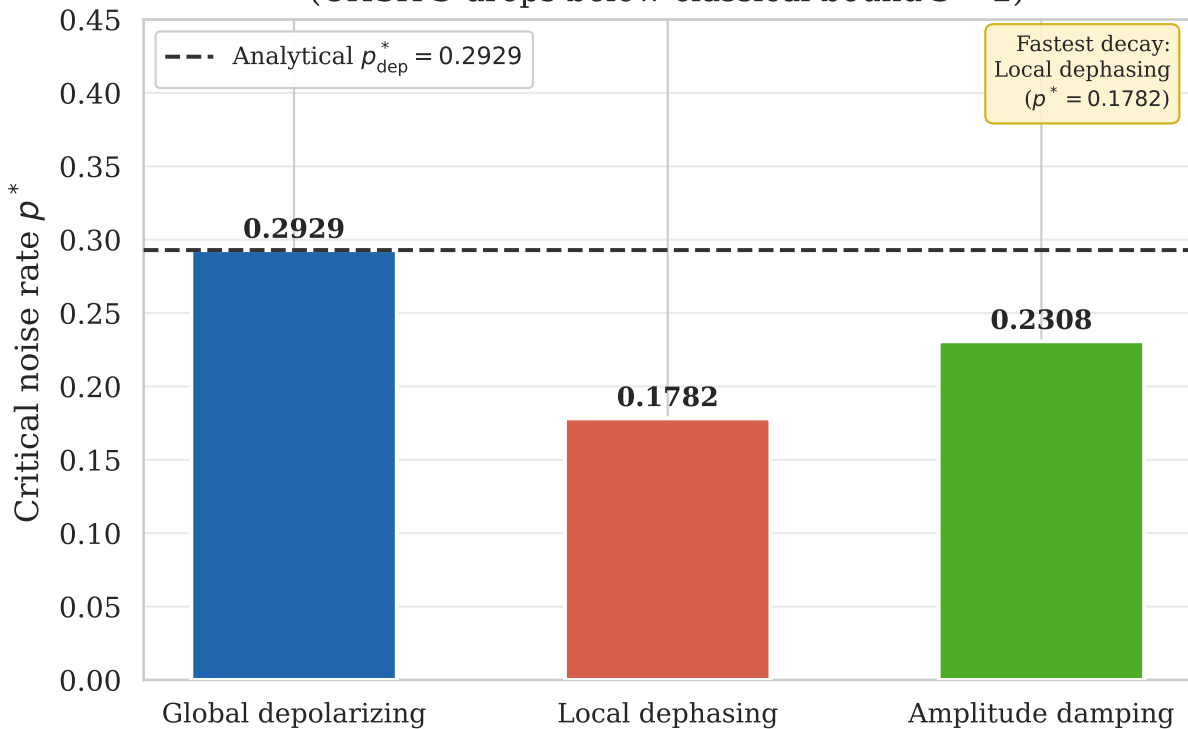
Noise Threshold p^* by Channel (CHSH S drops below classical bound S = 2 )
