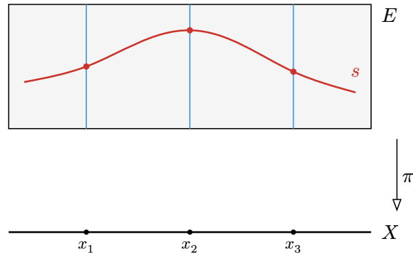
Figure 2: A real vector bundle \pi : E \rightarrow X . A section s picks one point s(x) in each fiber E_x ; the continuous sections form a C(X) -module.
