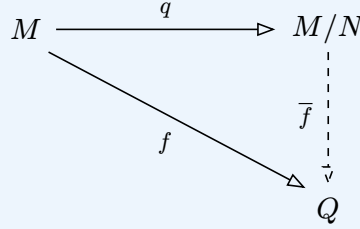
Figure 3: Universal property of M/N : any f : M \rightarrow Q with N \subseteq \ker f factors uniquely through the quotient.
