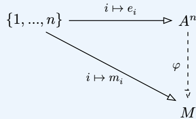
Figure 4: Universal property of A^n : any choice e_i \mapsto m_i of n elements of M extends uniquely to an A -linear map \varphi .
