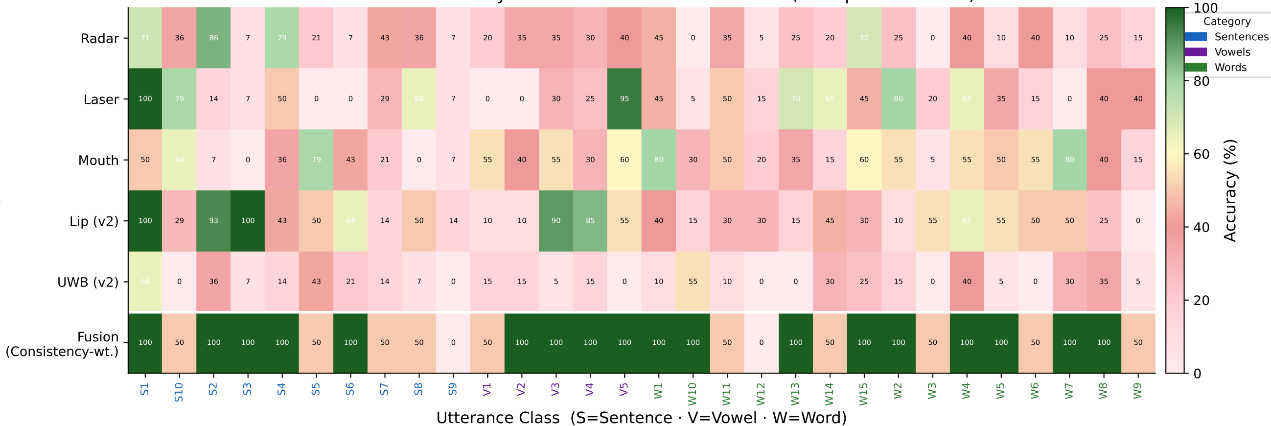
Per-Class Test Accuracy: Individual Modalities vs. Fusion (test speakers 19-20)
