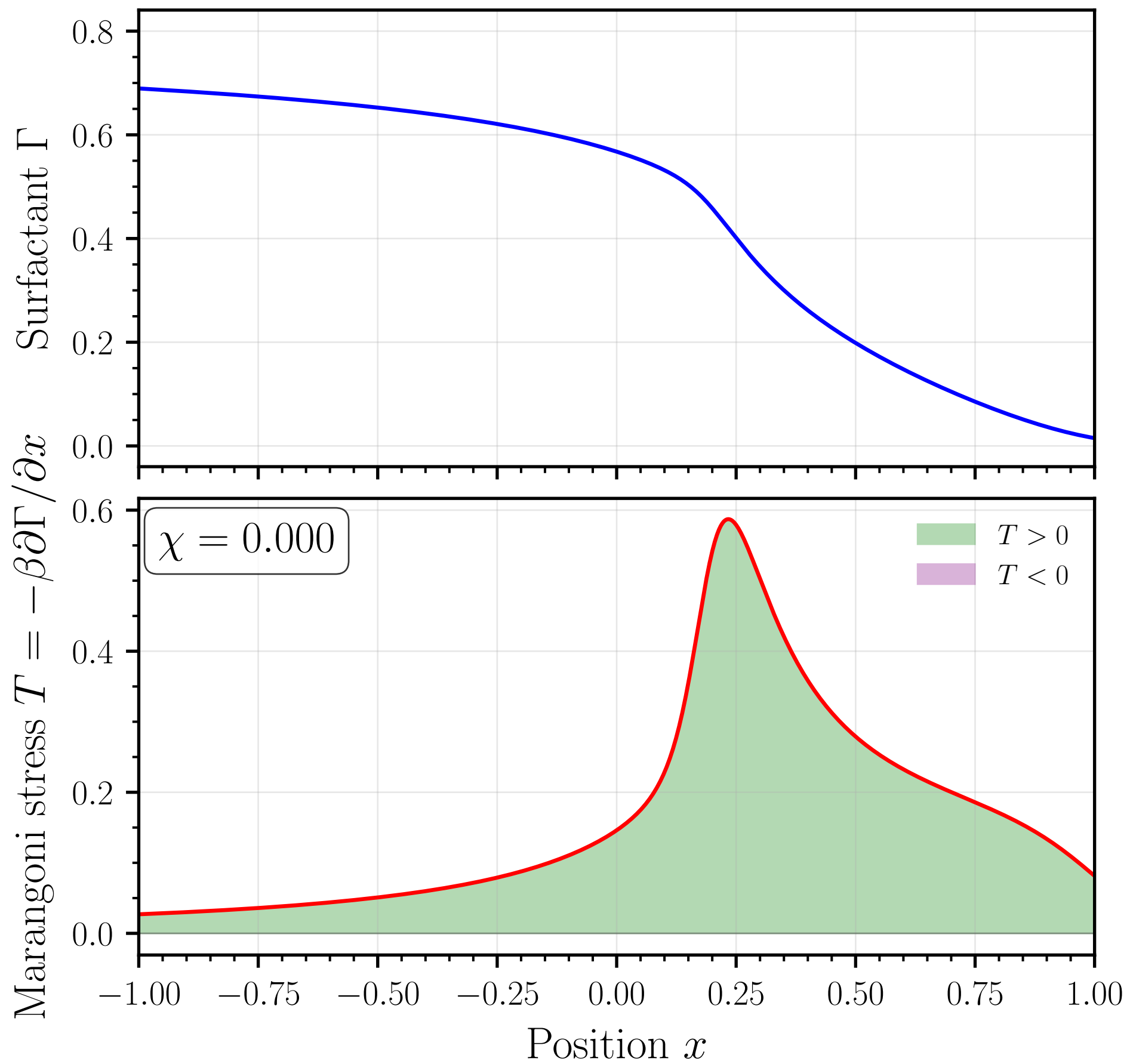
Surfactant and Marangoni Stress at t = 30.00
