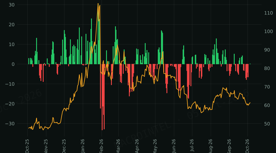
Silver · 5-Day Rate of Change (1 Year)
