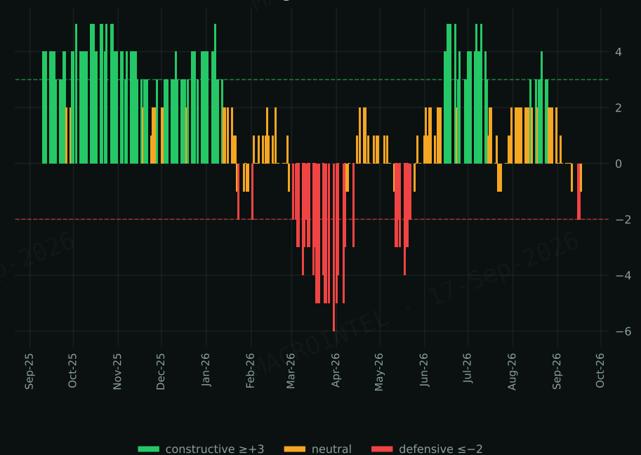
Net Score · Regime Ribbon (1 Year)
