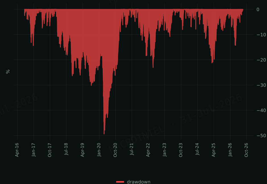
Midcap 100 · Drawdown from High
