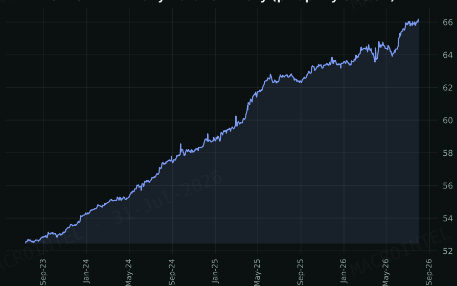
Gilt 5Y ETF · Daily Duration Proxy (px up = yields dn)
