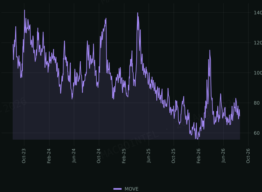
MOVE Index · US Rates Vol
