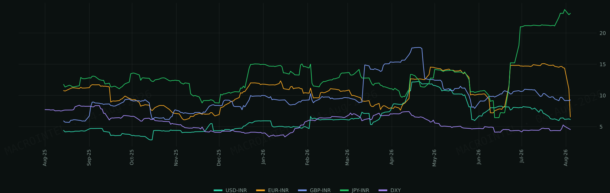
INR Complex · 30-Day Realized Volatility (1 Year)
