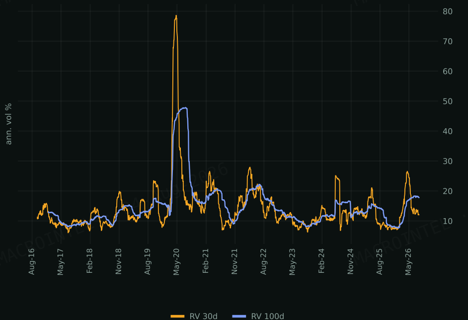
Sensex · Realized Volatility 30d vs 100d
