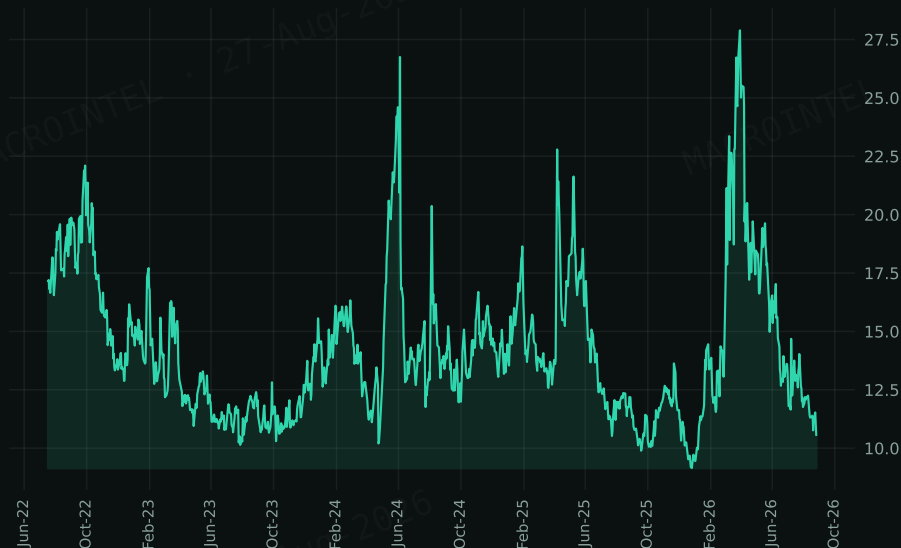
India VIX
