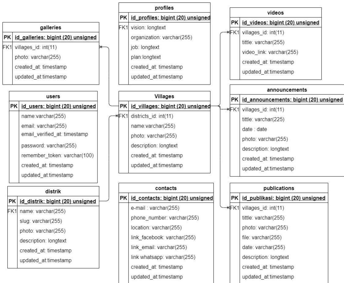
Gambar 16 Entity relationship diagram
