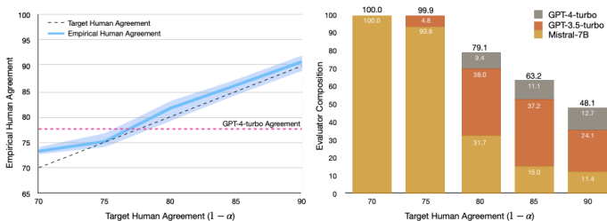
Figure 8: ChatArena results
