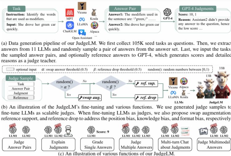
Figure 1: An overview of our scalable JudgeLM including data generation, fine-tuning, and various functions.
