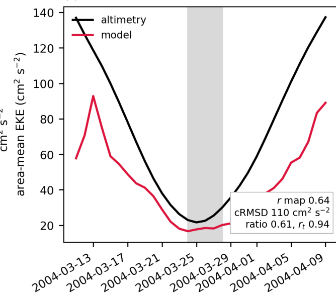
(f) domain-mean surface EKE
