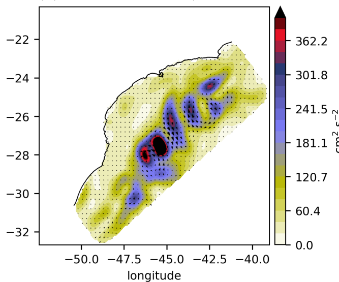
(e) model surface EKE, filtered
