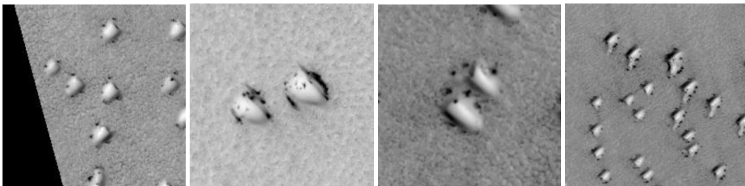
Crater
