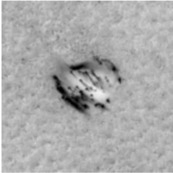
Bright Dune
