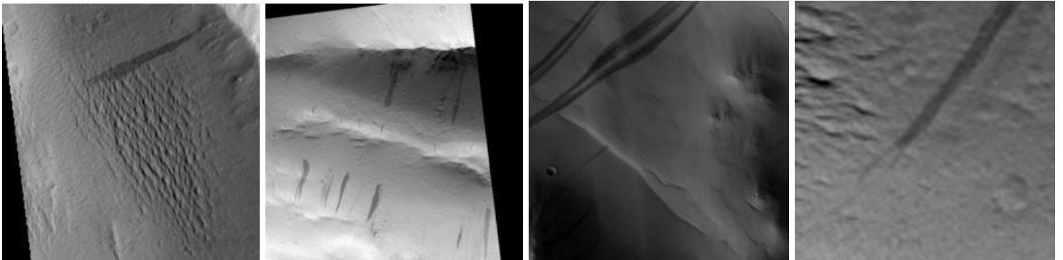
Spider
