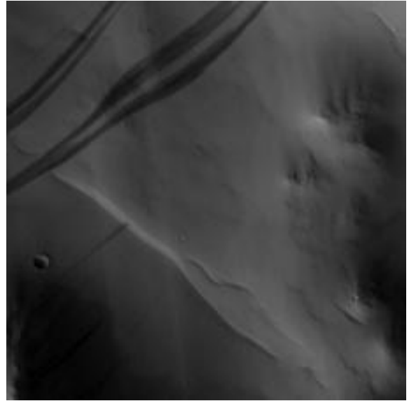
Slope Streak
