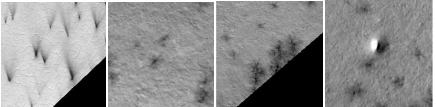
Swiss Cheese
