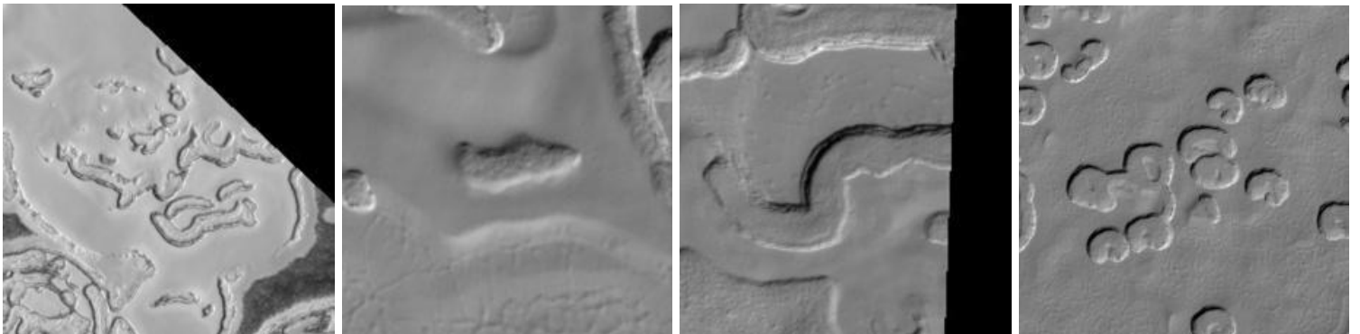
Swiss Cheese
