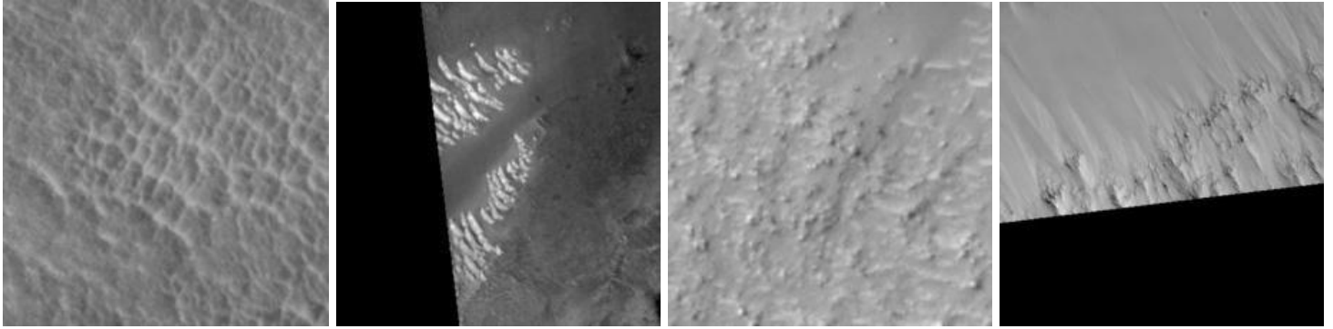
Slope Streak
