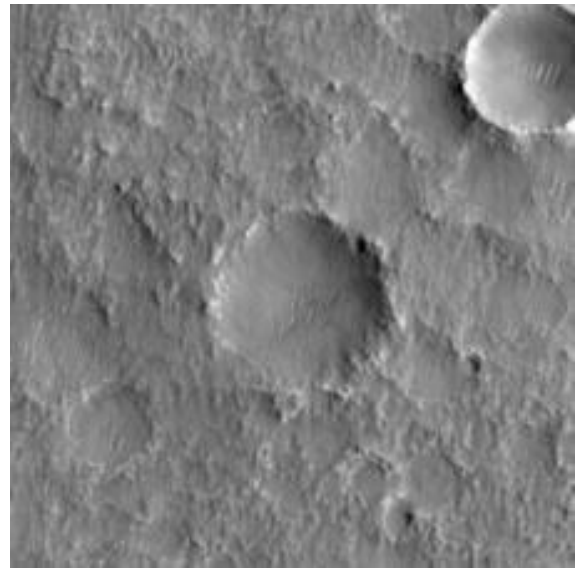
Crater
