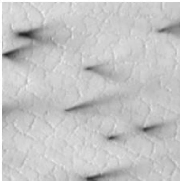
Spider
