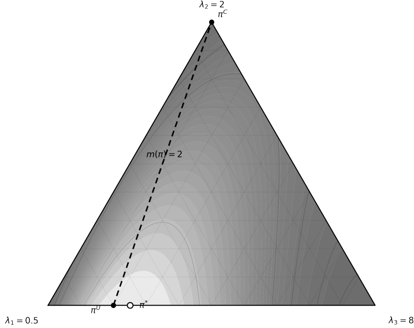
Figure 1: Belief simplex for the three-state baseline \lambda = (0.5, 2, 8)^\top . The grayscale field encodes the exact certainty-equivalent decision loss R_{\text{CE}}(\pi, 1) at the first learning-sensitive horizon. Five contour levels, one from each stable topological regime of the baseline loss surface, produce nine visible connected components with counts 1, 2, 3, 2, 1. The dashed segment is the fixed-mean fiber m(\pi) = 2 . Its endpoints \pi^C = (0, 1, 0) and \pi^U = (0.8, 0, 0.2) share the same current expected impact and, under the affine condition, the same unconditional future mean-impact path while differing in the value of future adaptation. The open marker \pi^* denotes the baseline global worst belief on the low/high support pair.
