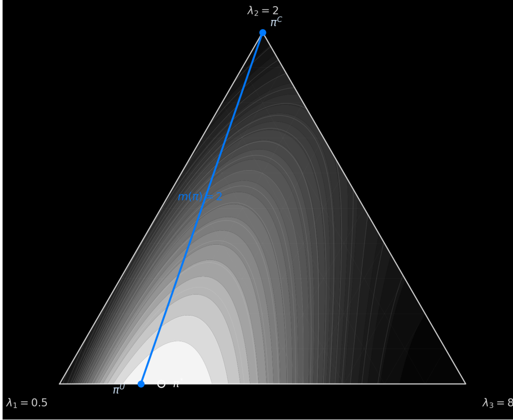
Figure 1: Belief simplex for the three-state baseline \lambda = (0.5, 2, 8)^\top . Each point in the triangle is a posterior belief over the three latent liquidity regimes. The grayscale field shows the normalized certainty-equivalent decision loss R_{\text{CE}}(\pi, 1) at the first learning-sensitive horizon. White curves are iso-loss contours. The blue segment is the fixed-mean fiber m(\pi) = 2 , along which all beliefs share the same current expected impact and, under the affine condition, the same unconditional future mean-impact path. The endpoints \pi^C = (0, 1, 0) and \pi^U = (0.8, 0, 0.2) therefore report the same liquidity estimate while differing in the value of future adaptation. The marker \pi^* denotes the baseline global worst belief on the low/high support pair.
