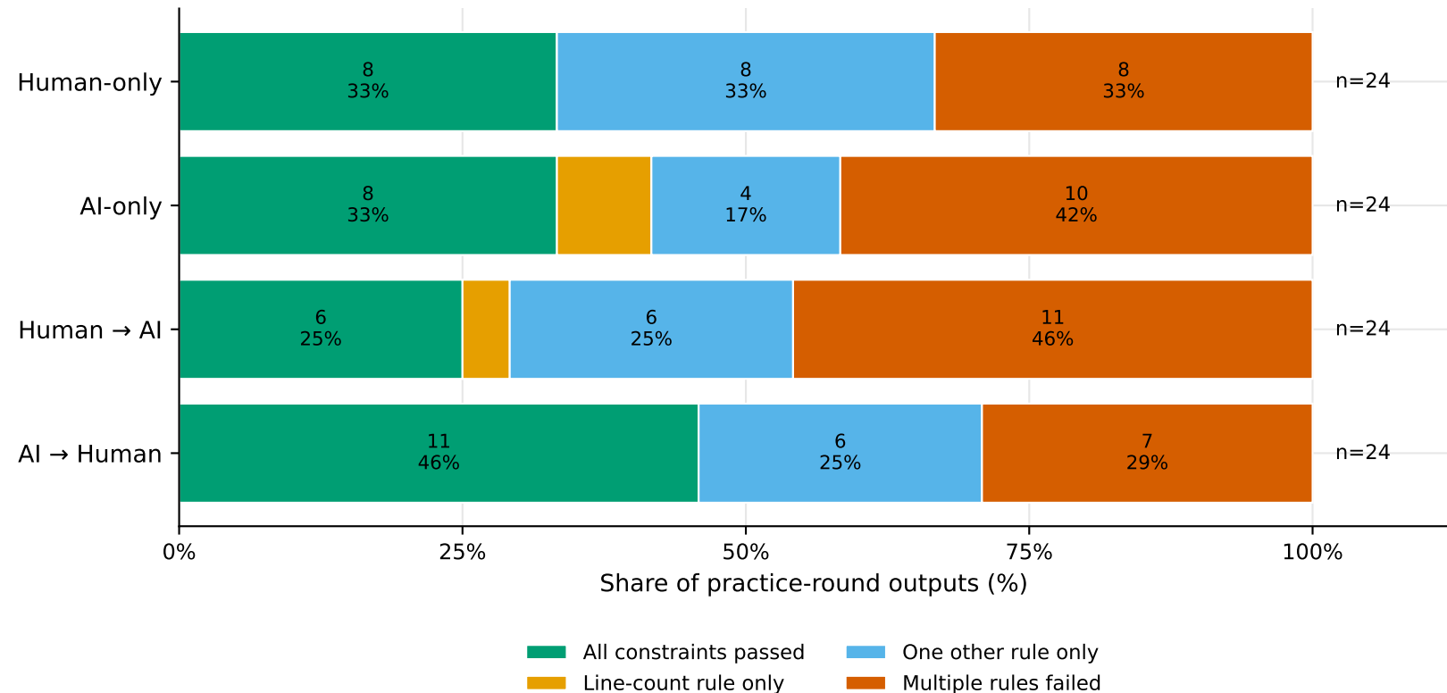
Constraint Failure Profiles by Workflow in Practice Rounds
