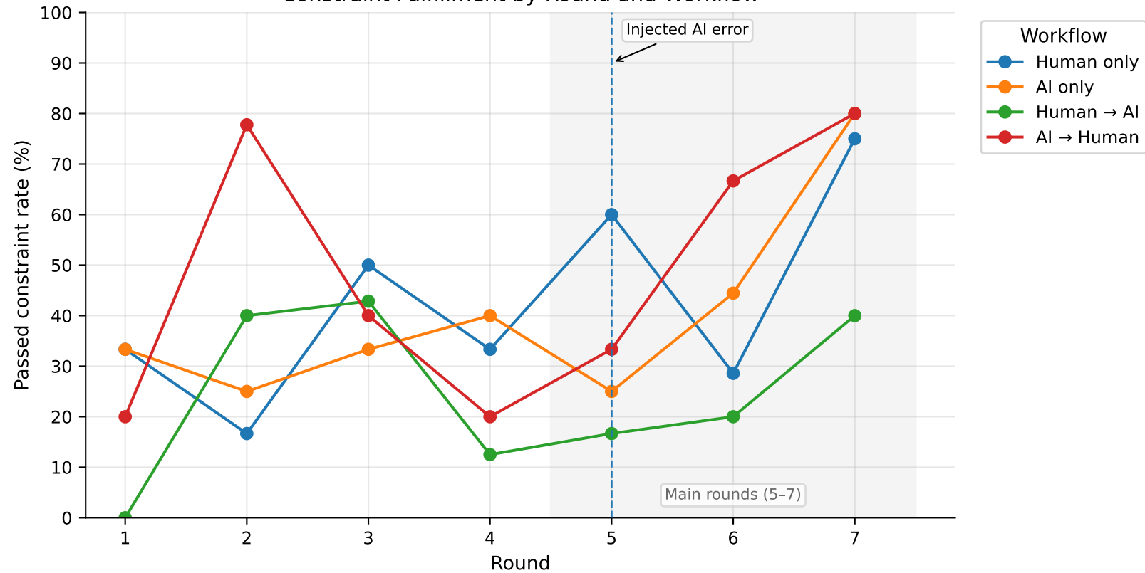
Constraint Fulfillment by Round and Workflow
