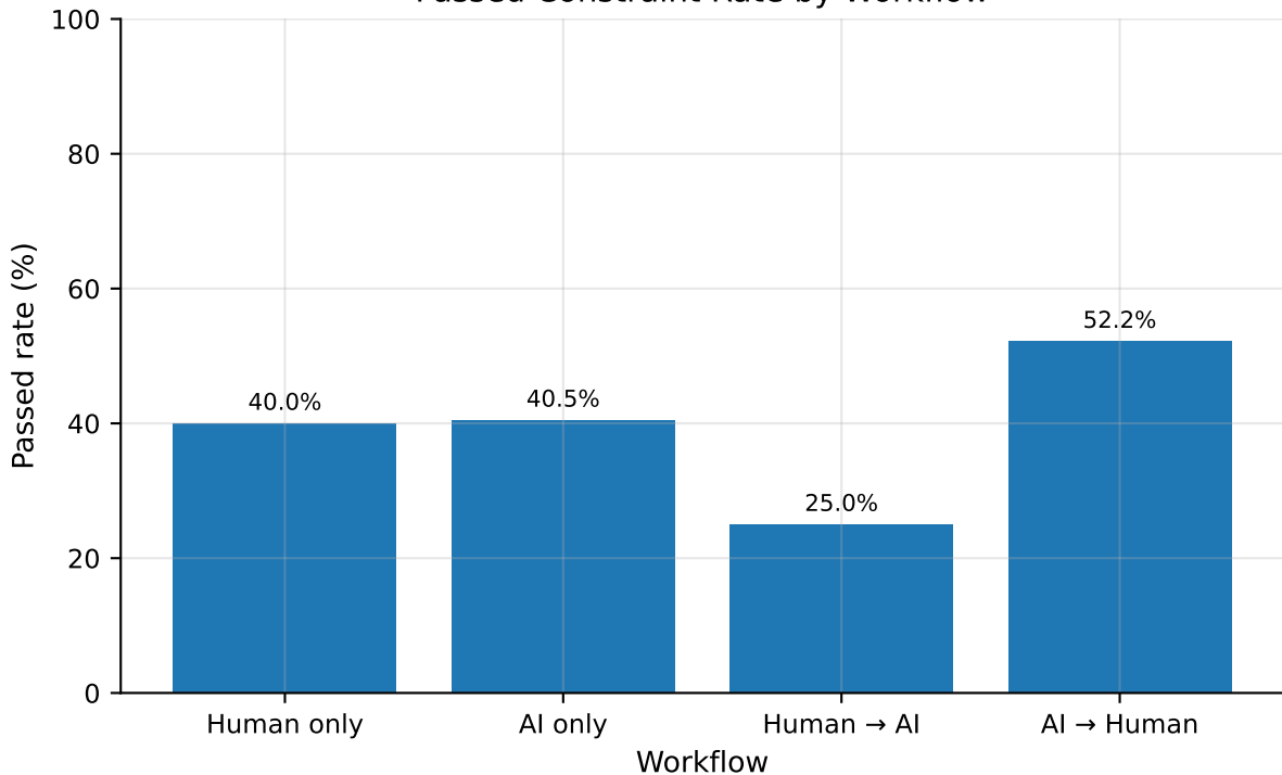
Passed Constraint Rate by Workflow
