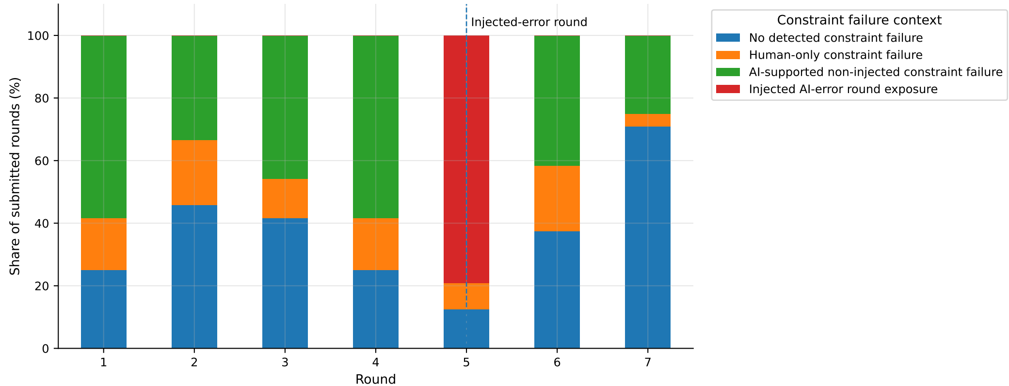
Constraint Failure Context over Rounds
