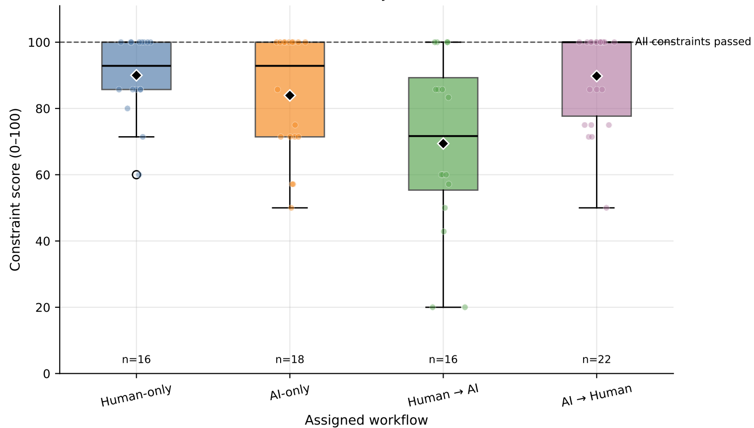
Constraint Score Distribution by Workflow in Main Rounds
