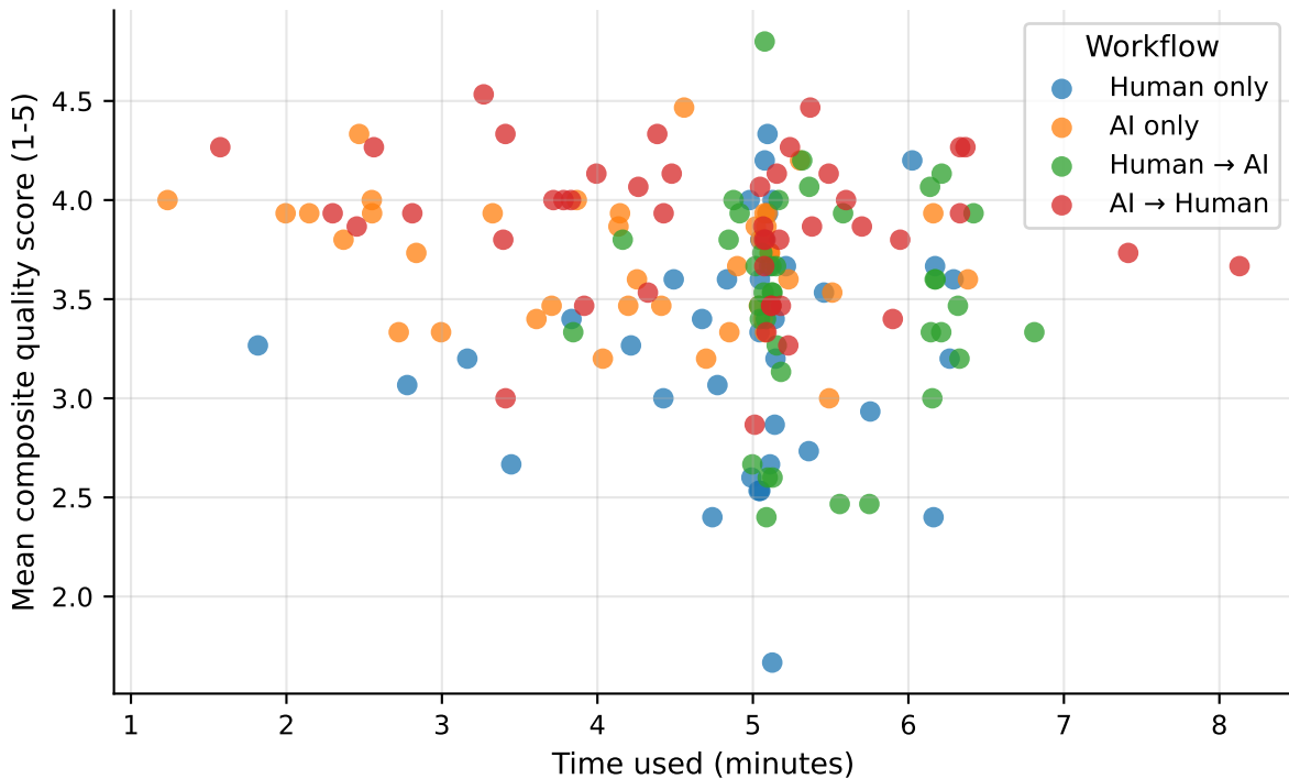
Output Composite Quality vs. Completion Time
