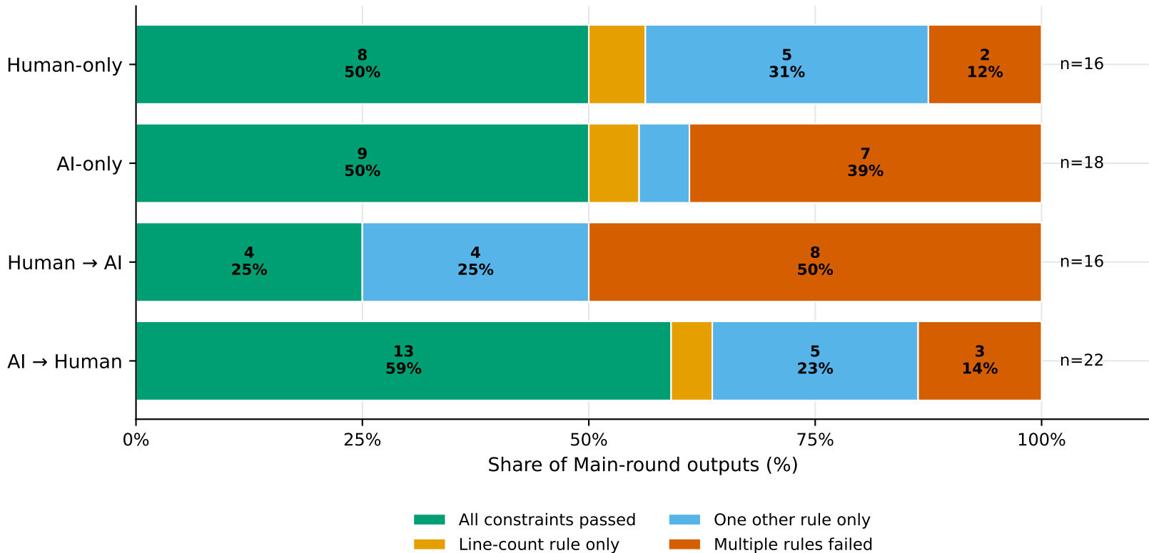
Constraint Failure Profiles by Workflow in Main Rounds
