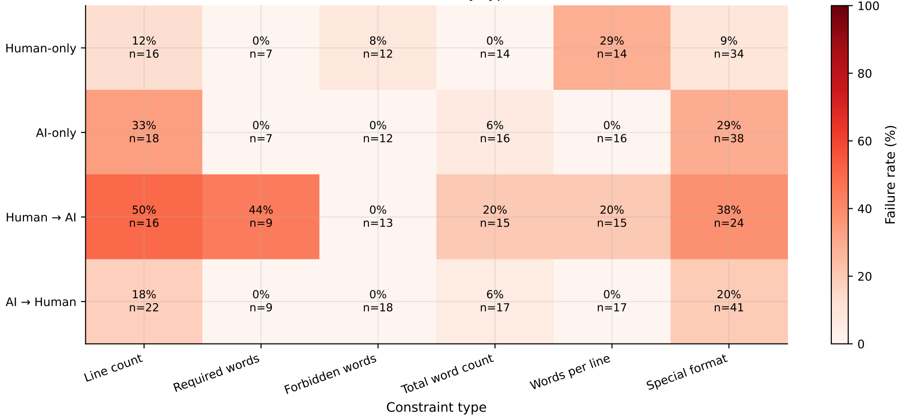
Constraint Failure Breakdown by Type in Main Rounds
