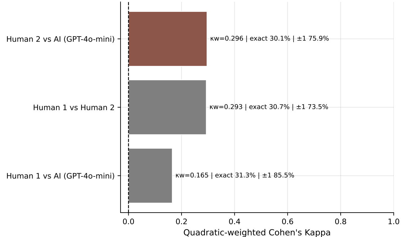
Pairwise Agreement Between Evaluators
