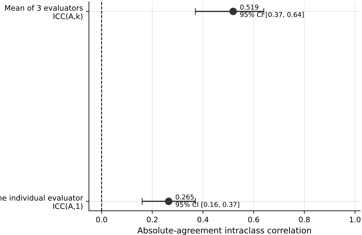
Reliability of the Overall-Quality Score
